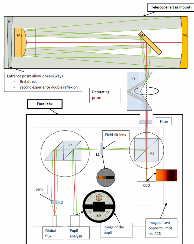
Fig. 4 MISOLFA optical design. See text for details.
