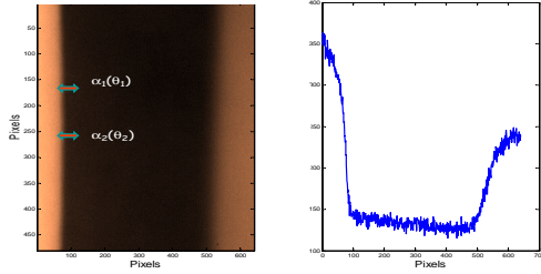
Fig. 6 Image sample from the MISOLFA monitor (left) and horizontal cut (right). Arrows illustrate the motions used to compute the transverse covariance between to angular positions (see text).
